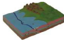
F04 Convergent Plate Boundaries
