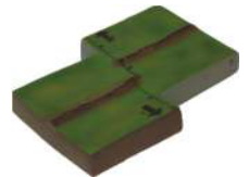
F06 Transform Plate Boundaries
