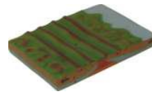
F05 Divergent Plate Boundaries
