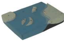
F03 Ice Sheet & Icebergs
