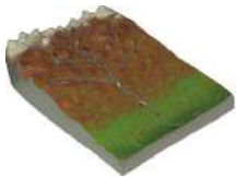
F01 Collecting River system
